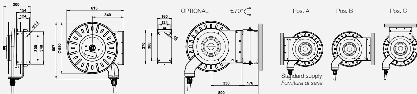
BGDX Dimensions (mm) / Dimensioni (mm)
